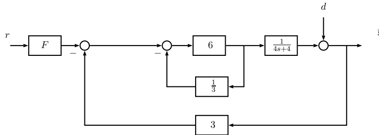
Figure 1: Blockdiagram
